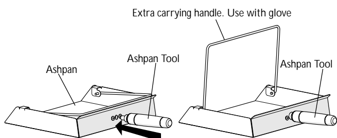
Fig.4.Ash Removal
